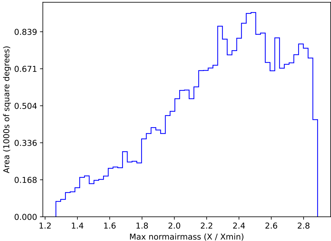
early_u_fpextra2.0_v3.4_10yrs All sky all bands: Max normairmass
