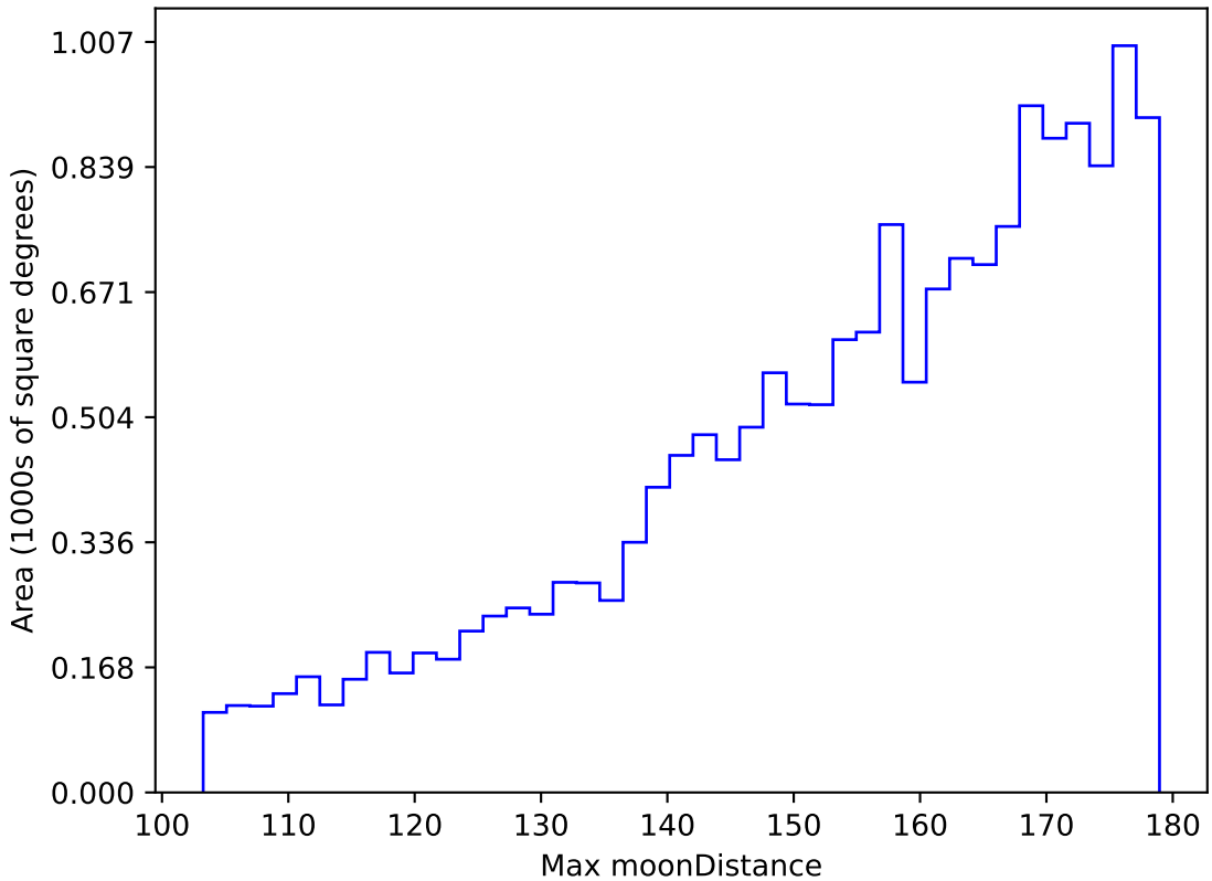
early_u_fpextra2.0_v3.4_10yrs WFD z band: Max moonDistance
