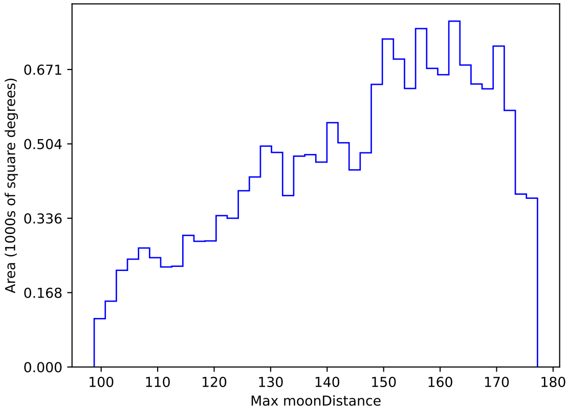
early_u_fpextra2.0_v3.4_10yrs WFD y band: Max moonDistance
