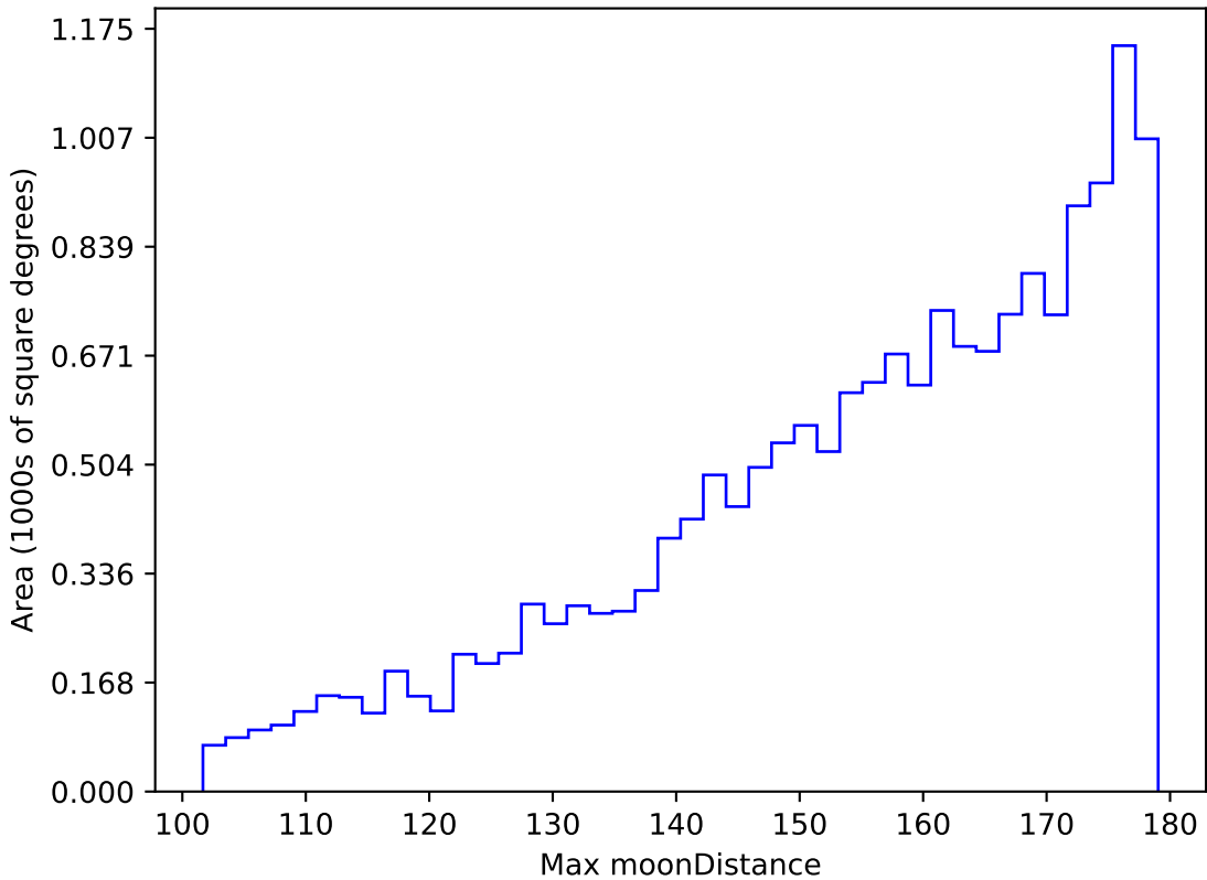
early_u_fpextra2.0_v3.4_10yrs WFD u band: Max moonDistance
