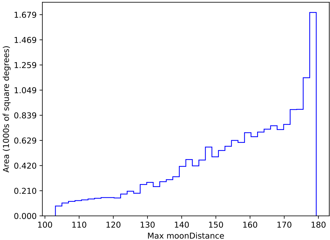
early_u_fpextra2.0_v3.4_10yrs WFD r band: Max moonDistance
