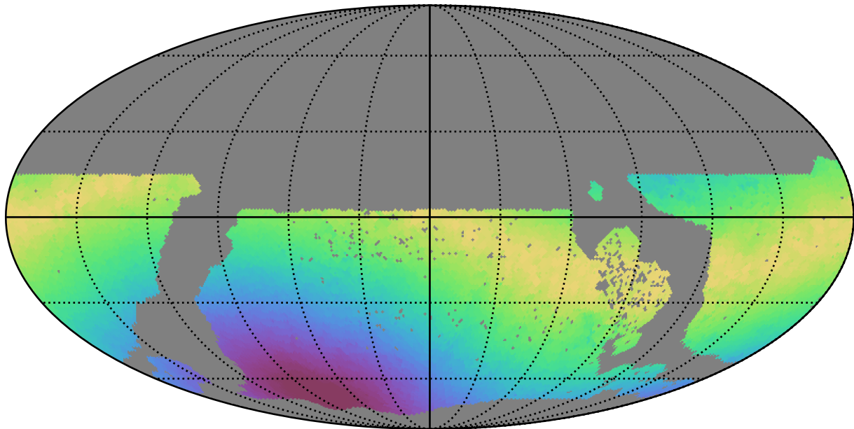
early_u_fpextra2.0_v3.4_10yrs WFD g band: Max moonDistance
