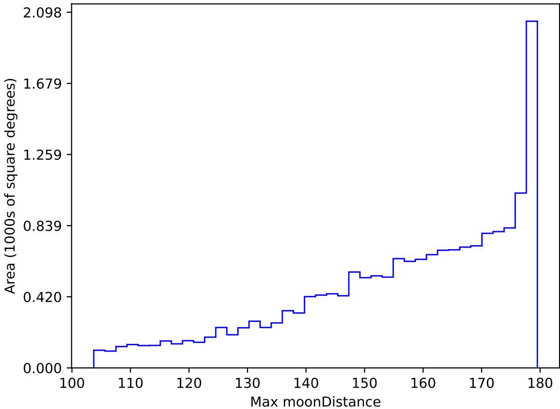
early_u_fpextra2.0_v3.4_10yrs WFD all bands: Max moonDistance
