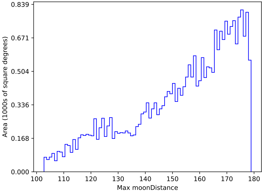
early_u_fpextra2.0_v3.4_10yrs All sky z band: Max moonDistance
