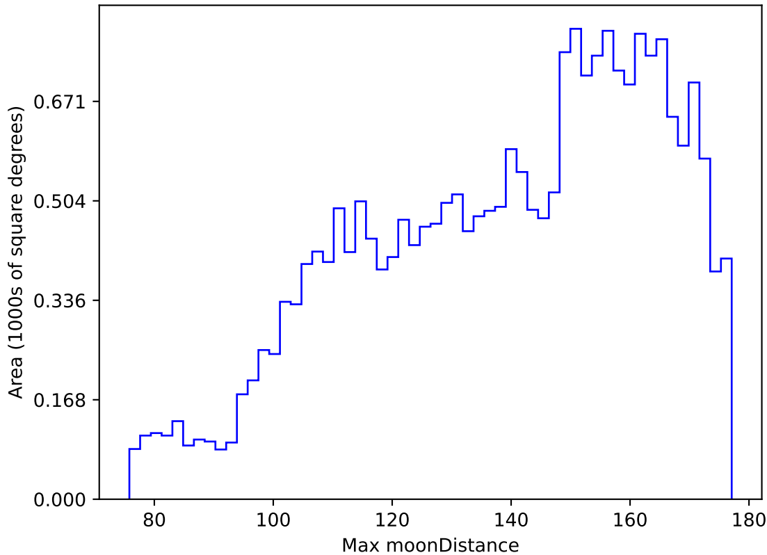
early_u_fpextra2.0_v3.4_10yrs All sky y band: Max moonDistance
