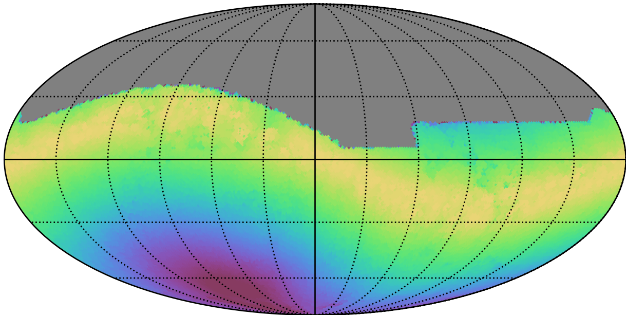
early_u_fpextra2.0_v3.4_10yrs All sky r band: Max moonDistance
