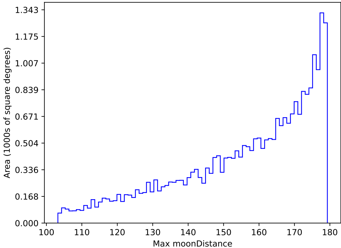
early_u_fpextra2.0_v3.4_10yrs All sky r band: Max moonDistance
