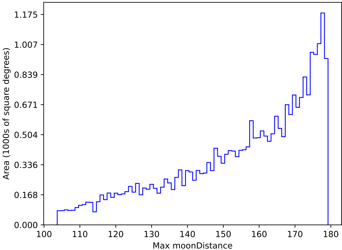
early_u_fpextra2.0_v3.4_10yrs All sky i band: Max moonDistance
