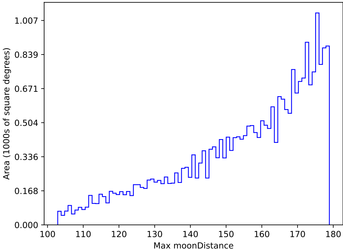
early_u_fpextra2.0_v3.4_10yrs All sky g band: Max moonDistance
