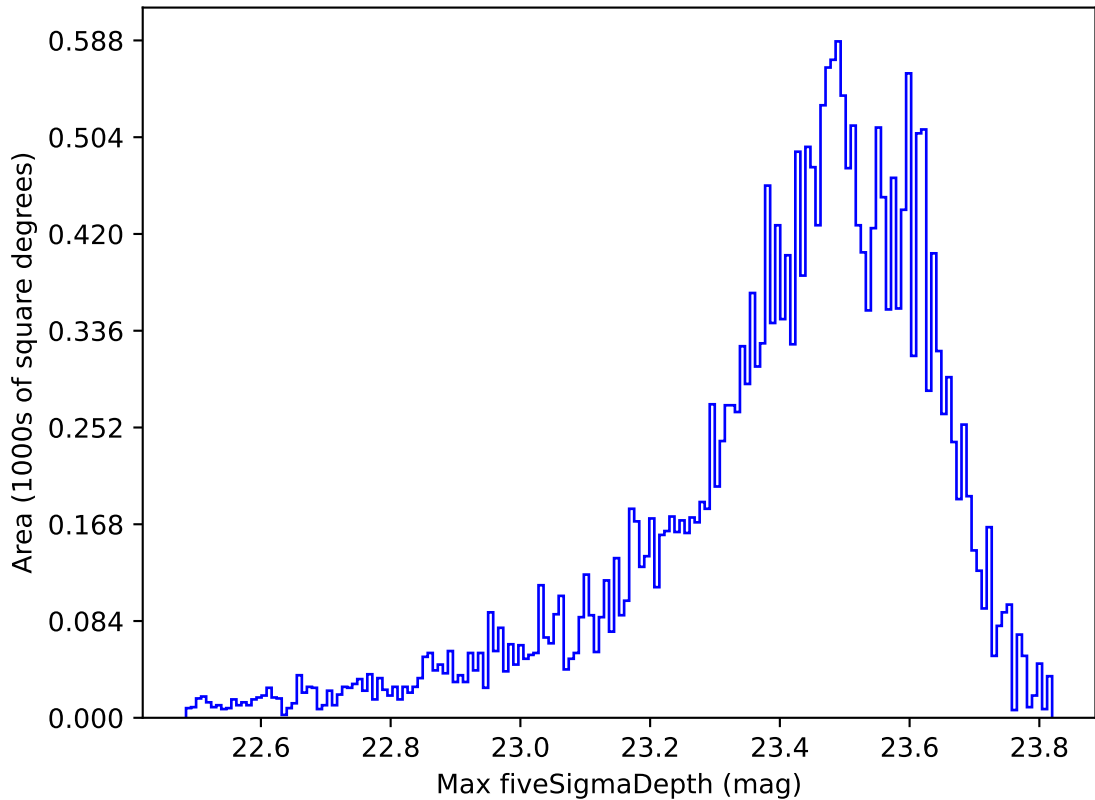
early_u_fpextra2.0_v3.4_10yrs Yr 1 z band: Max fiveSigmaDepth
