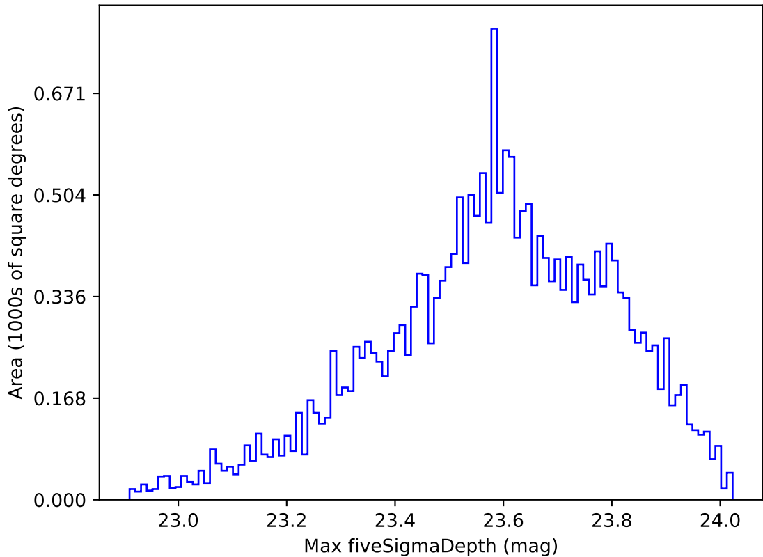
early_u_fpextra2.0_v3.4_10yrs Yr 1 u band: Max fiveSigmaDepth
