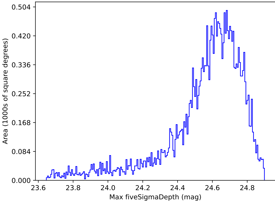
early_u_fpextra2.0_v3.4_10yrs Yr 1 r band: Max fiveSigmaDepth
