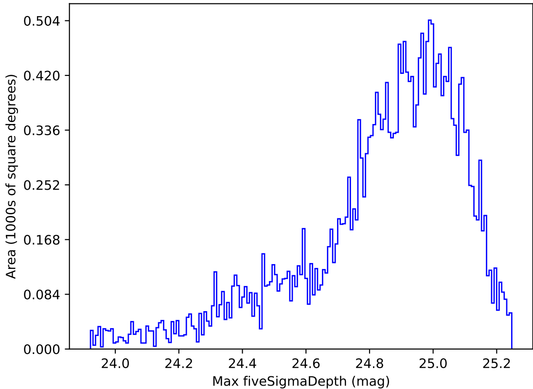
early_u_fpextra2.0_v3.4_10yrs Yr 1 g band: Max fiveSigmaDepth
