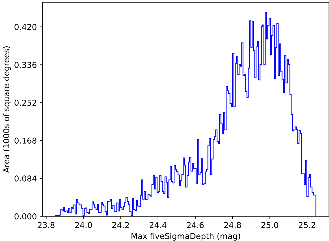
early_u_fpextra2.0_v3.4_10yrs Yr 1 all bands: Max fiveSigmaDepth
