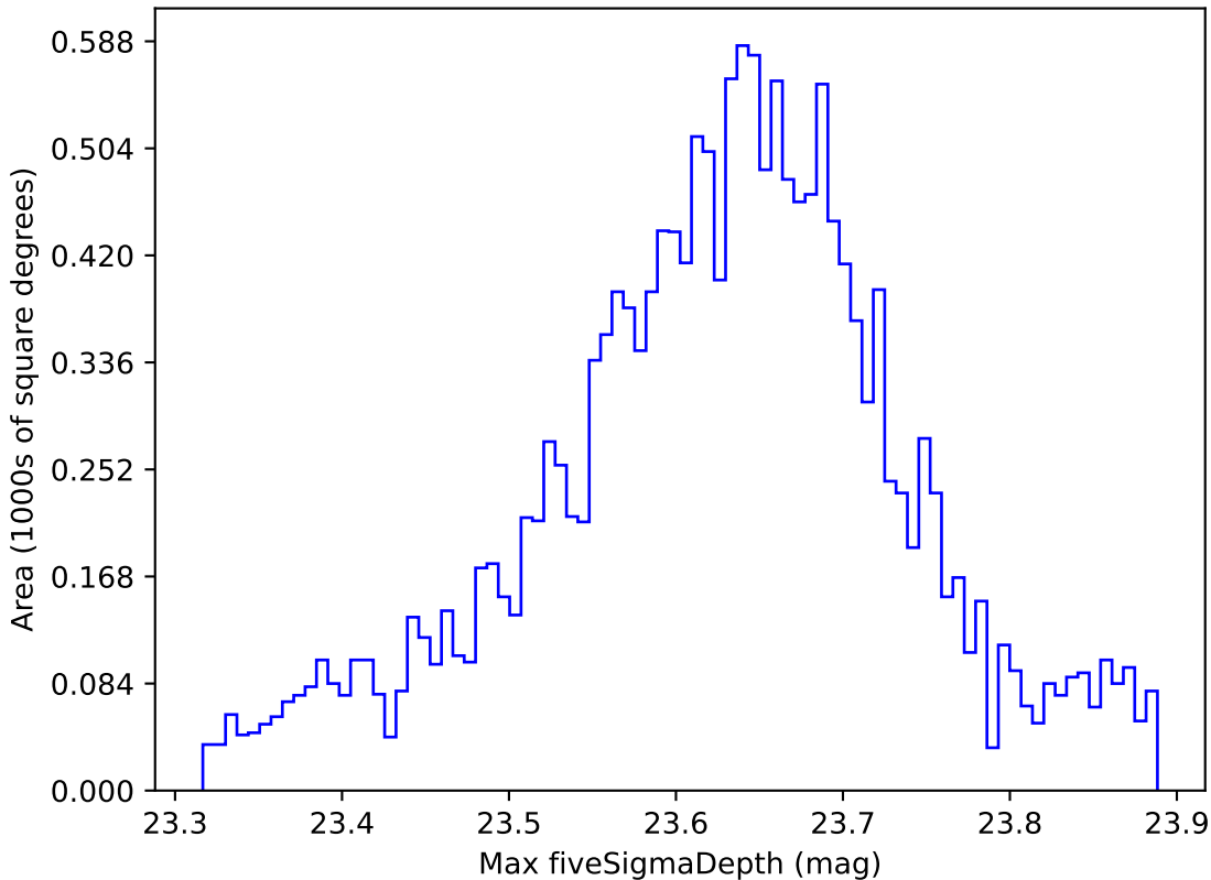
early_u_fpextra2.0_v3.4_10yrs WFD z band: Max fiveSigmaDepth
