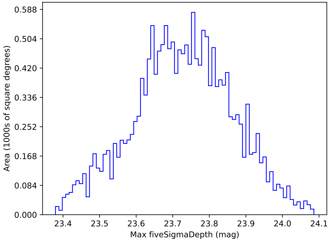
early_u_fpextra2.0_v3.4_10yrs WFD u band: Max fiveSigmaDepth
