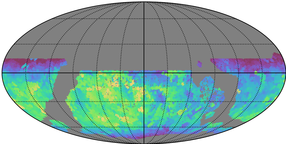
early_u_fpextra2.0_v3.4_10yrs WFD r band: Max fiveSigmaDepth
