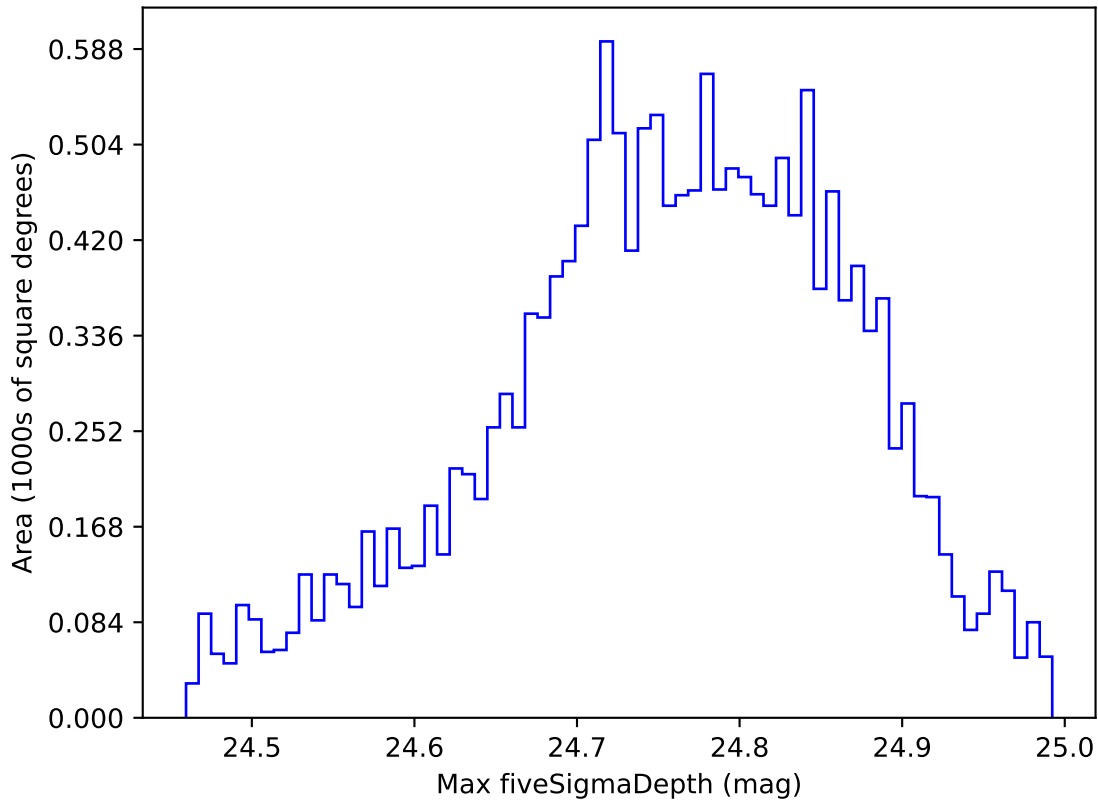
early_u_fpextra2.0_v3.4_10yrs WFD r band: Max fiveSigmaDepth
