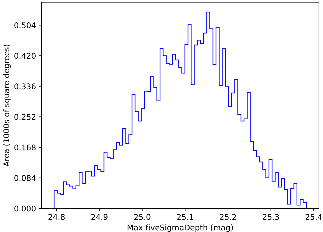
early_u_fpextra2.0_v3.4_10yrs WFD g band: Max fiveSigmaDepth
