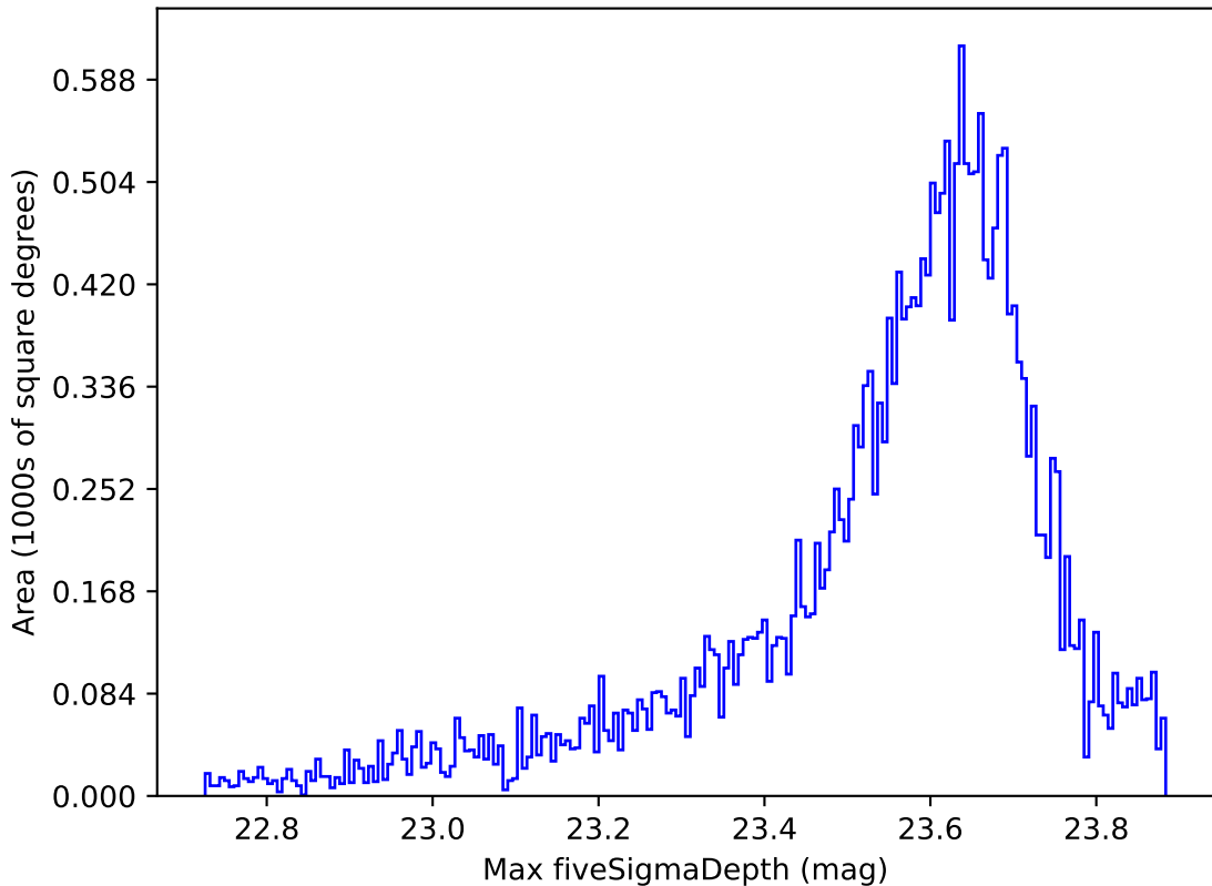
early_u_fpextra2.0_v3.4_10yrs All sky z band: Max fiveSigmaDepth
