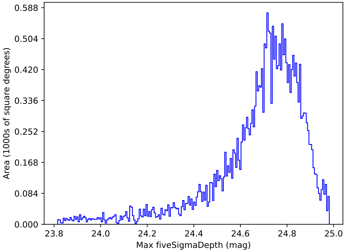
early_u_fpextra2.0_v3.4_10yrs All sky r band: Max fiveSigmaDepth
