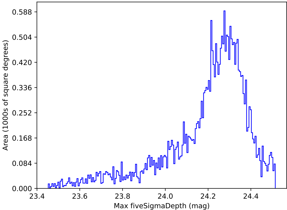
early_u_fpextra2.0_v3.4_10yrs All sky i band: Max fiveSigmaDepth
