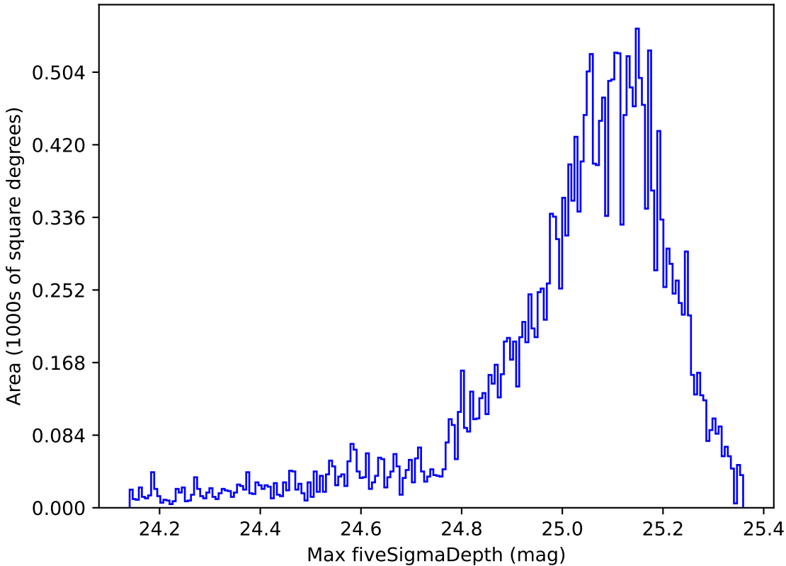
early_u_fpextra2.0_v3.4_10yrs All sky g band: Max fiveSigmaDepth
