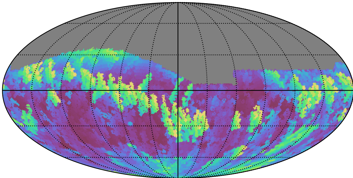
early_u_fpextra2.0_v3.4_10yrs Yr 1 z band: Max airmass
