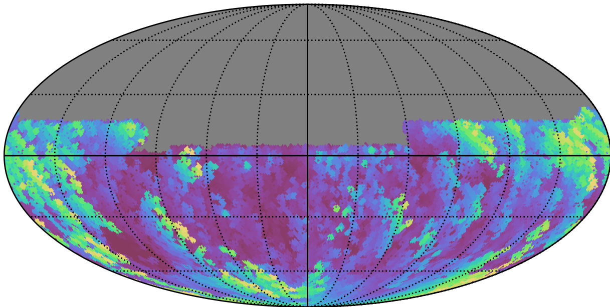
early_u_fpextra2.0_v3.4_10yrs Yr 1 y band: Max airmass
