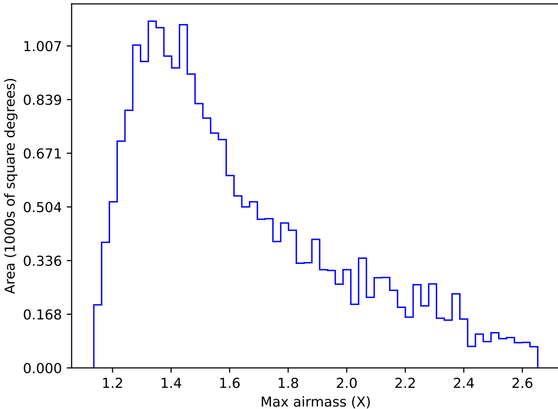
early_u_fpextra2.0_v3.4_10yrs Yr 1 y band: Max airmass
