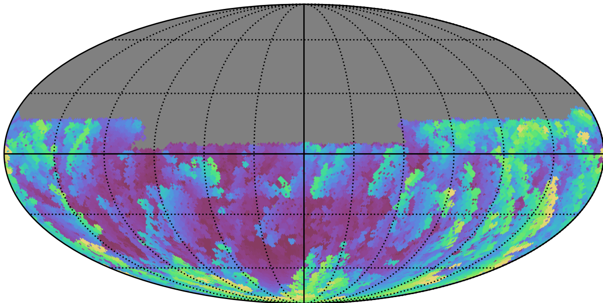
early_u_fpextra2.0_v3.4_10yrs Yr 1 u band: Max airmass
