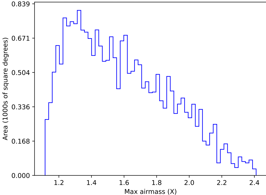
early_u_fpextra2.0_v3.4_10yrs Yr 1 u band: Max airmass
