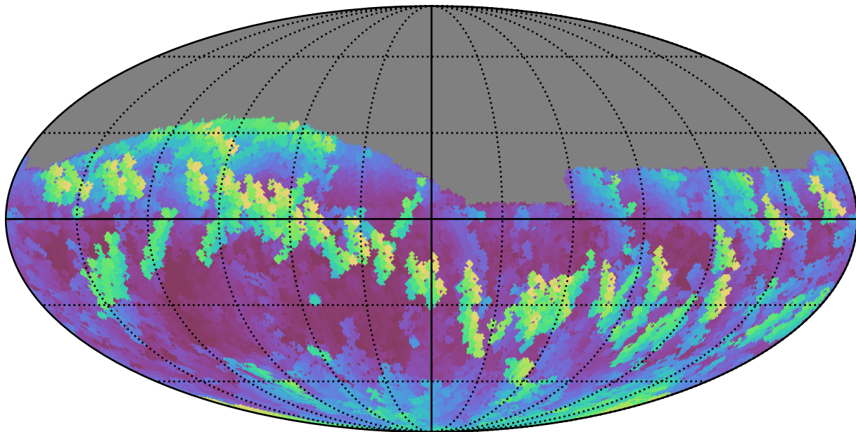
early_u_fpextra2.0_v3.4_10yrs Yr 1 i band: Max airmass
