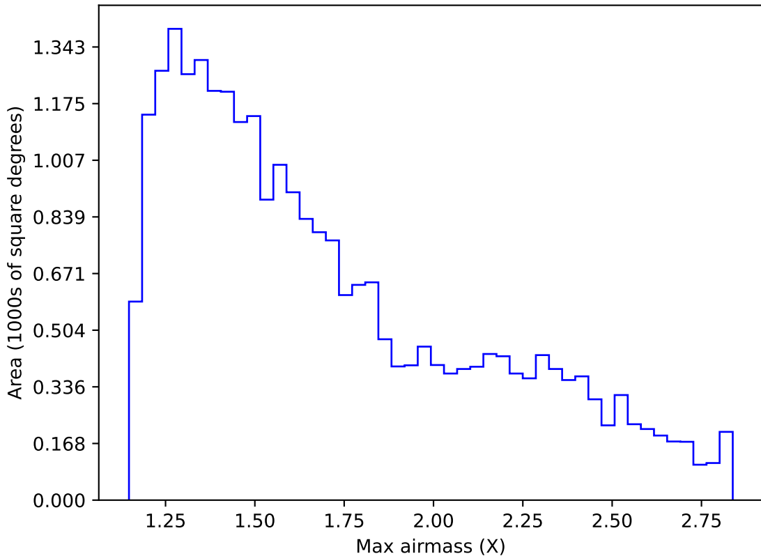
early_u_fpextra2.0_v3.4_10yrs Yr 1 i band: Max airmass
