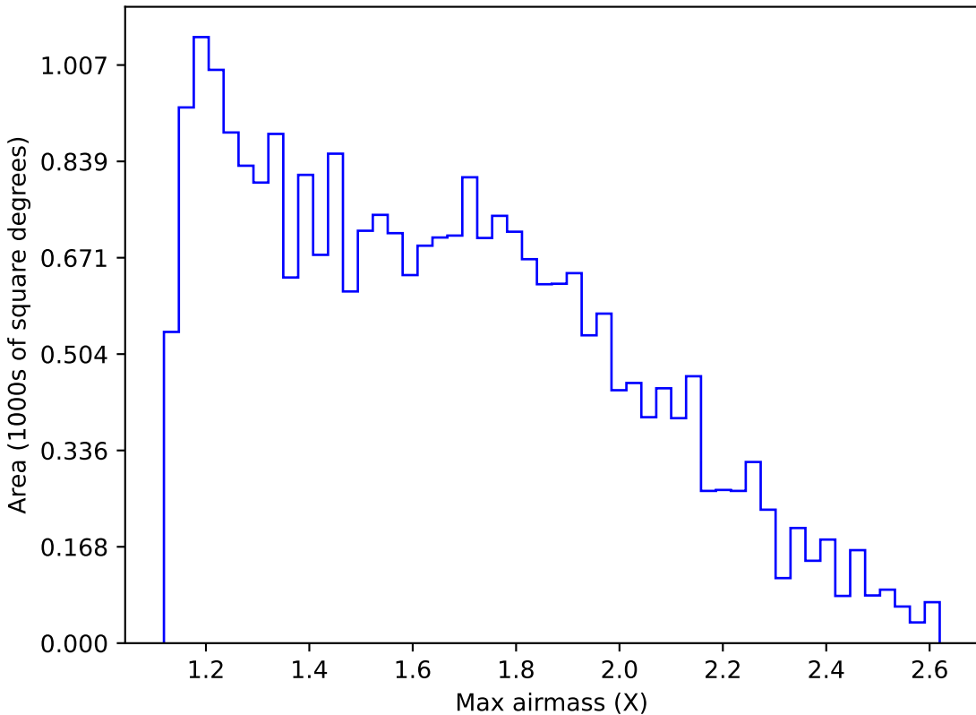
early_u_fpextra2.0_v3.4_10yrs Yr 1 g band: Max airmass
