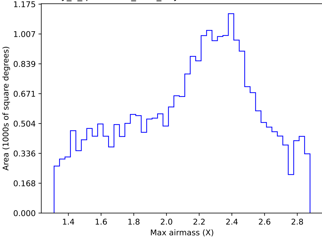
early_u_fpextra2.0_v3.4_10yrs Yr 1 all bands: Max airmass
