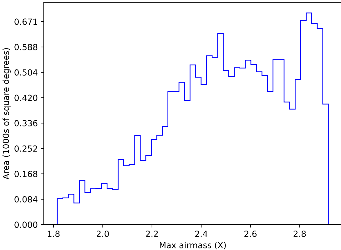
early_u_fpextra2.0_v3.4_10yrs WFD z band: Max airmass
