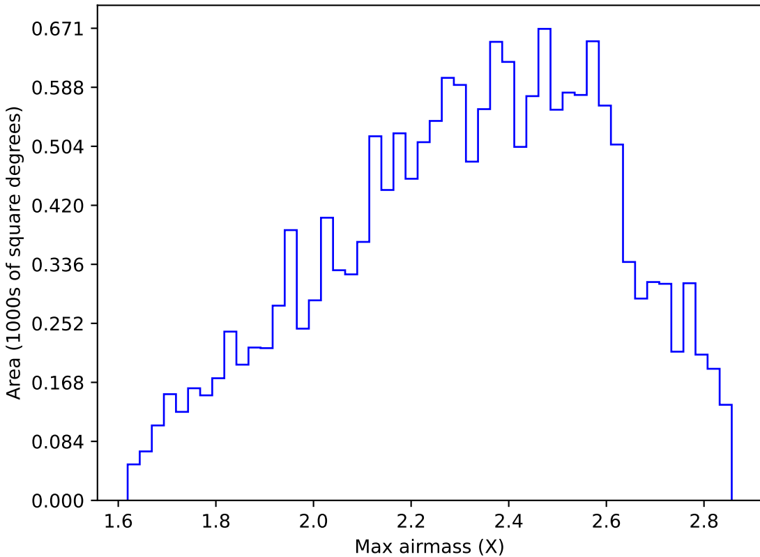
early_u_fpextra2.0_v3.4_10yrs WFD y band: Max airmass
