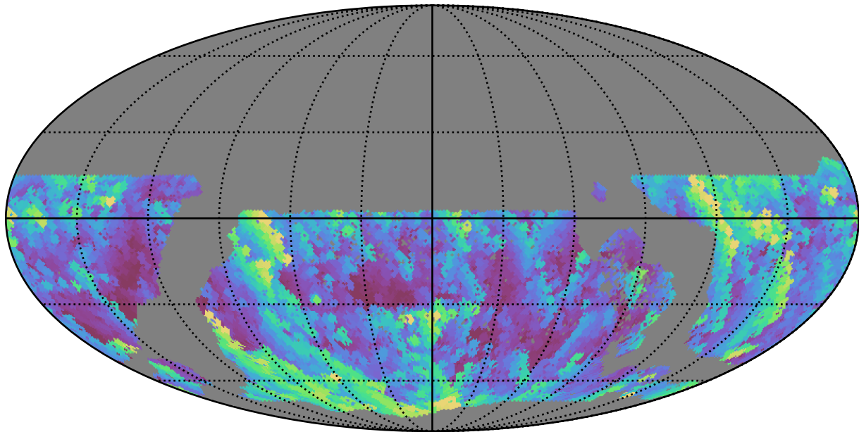
early_u_fpextra2.0_v3.4_10yrs WFD u band: Max airmass
