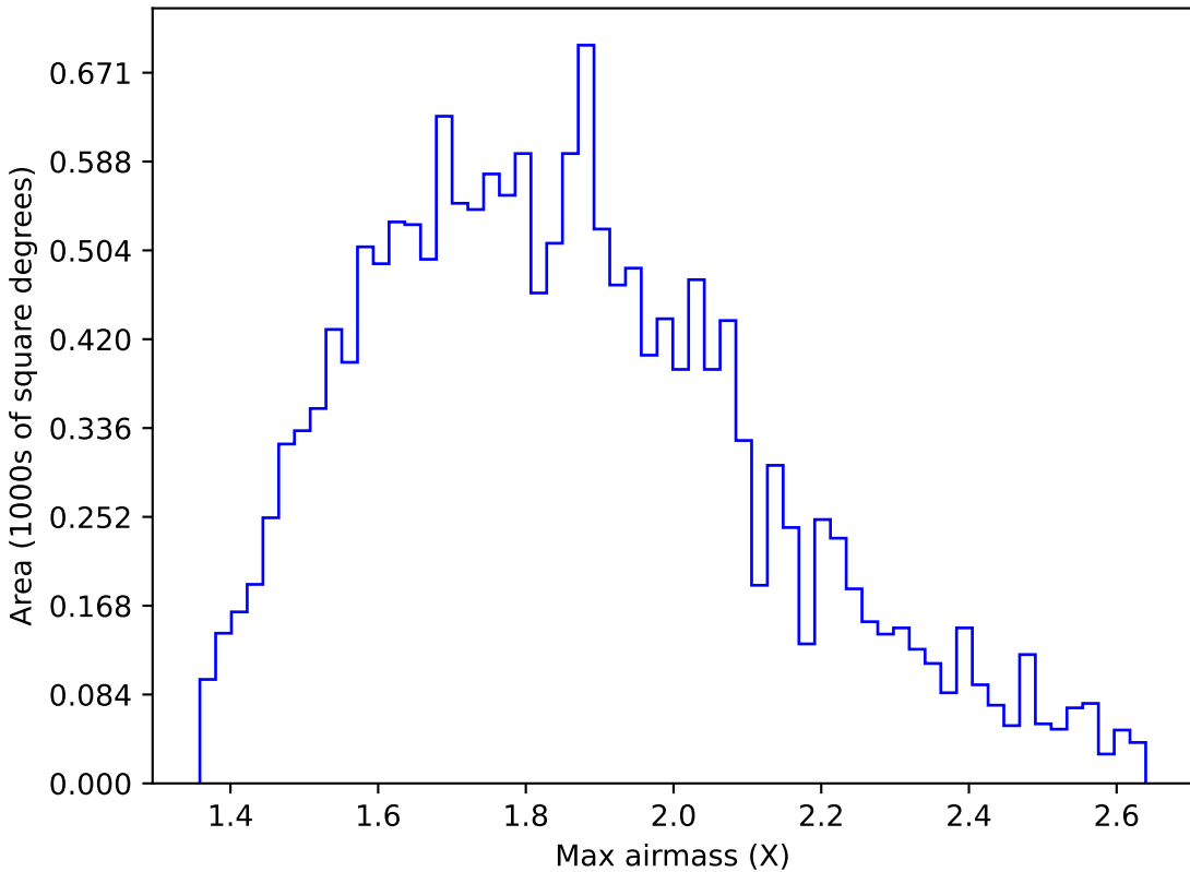
early_u_fpextra2.0_v3.4_10yrs WFD u band: Max airmass
