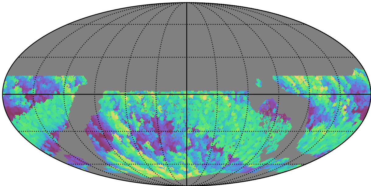
early_u_fpextra2.0_v3.4_10yrs WFD r band: Max airmass
