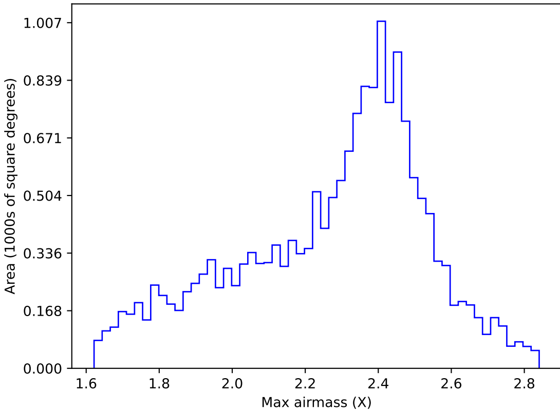
early_u_fpextra2.0_v3.4_10yrs WFD r band: Max airmass
