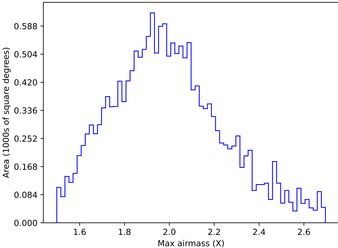
early_u_fpextra2.0_v3.4_10yrs WFD g band: Max airmass
