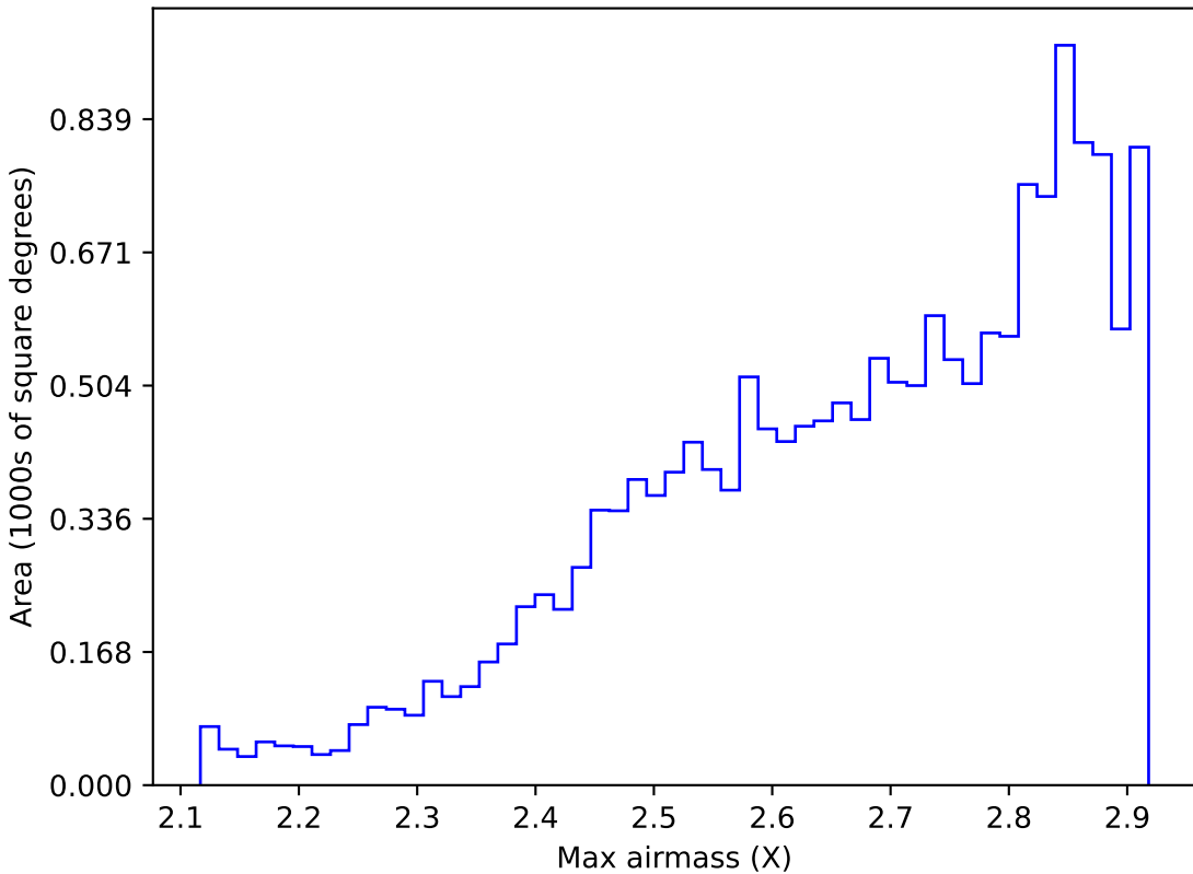
early_u_fpextra2.0_v3.4_10yrs WFD all bands: Max airmass
