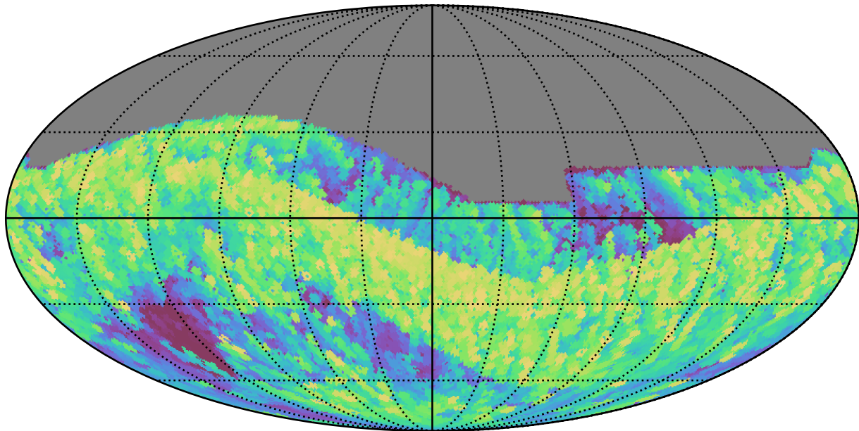
early_u_fpextra2.0_v3.4_10yrs All sky z band: Max airmass
