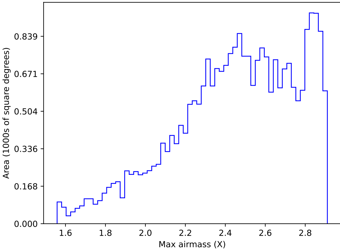
early_u_fpextra2.0_v3.4_10yrs All sky z band: Max airmass
