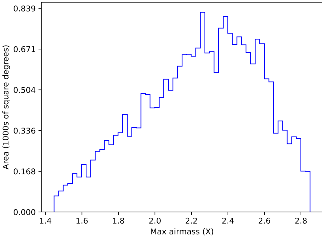
early_u_fpextra2.0_v3.4_10yrs All sky y band: Max airmass
