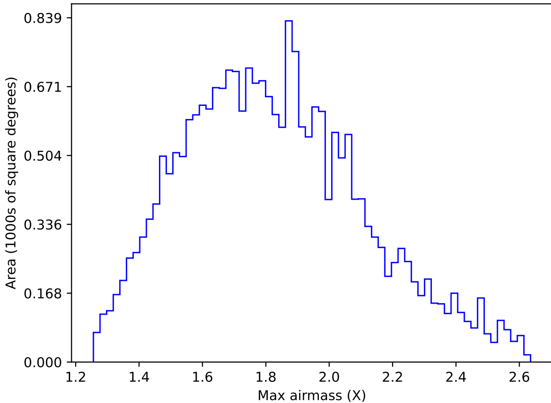
early_u_fpextra2.0_v3.4_10yrs All sky u band: Max airmass
