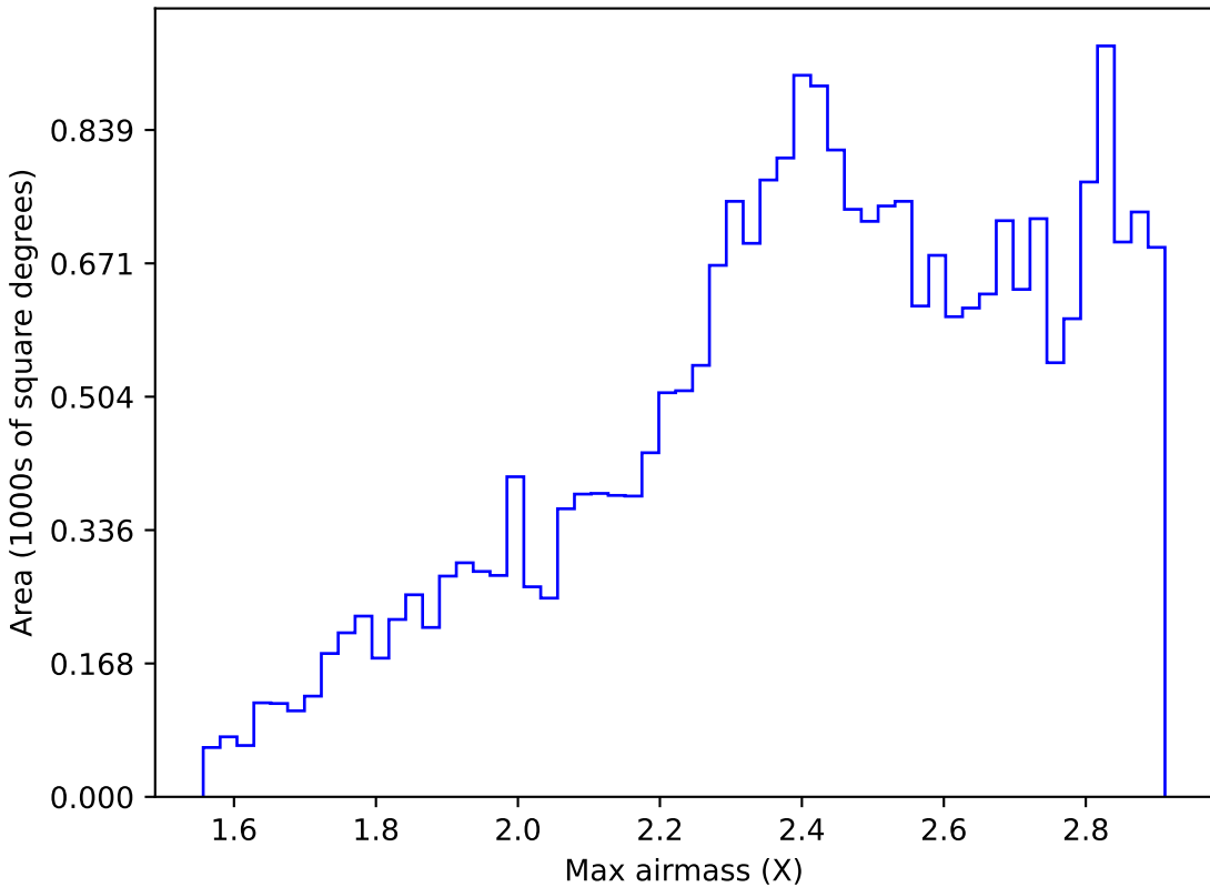
early_u_fpextra2.0_v3.4_10yrs All sky i band: Max airmass
