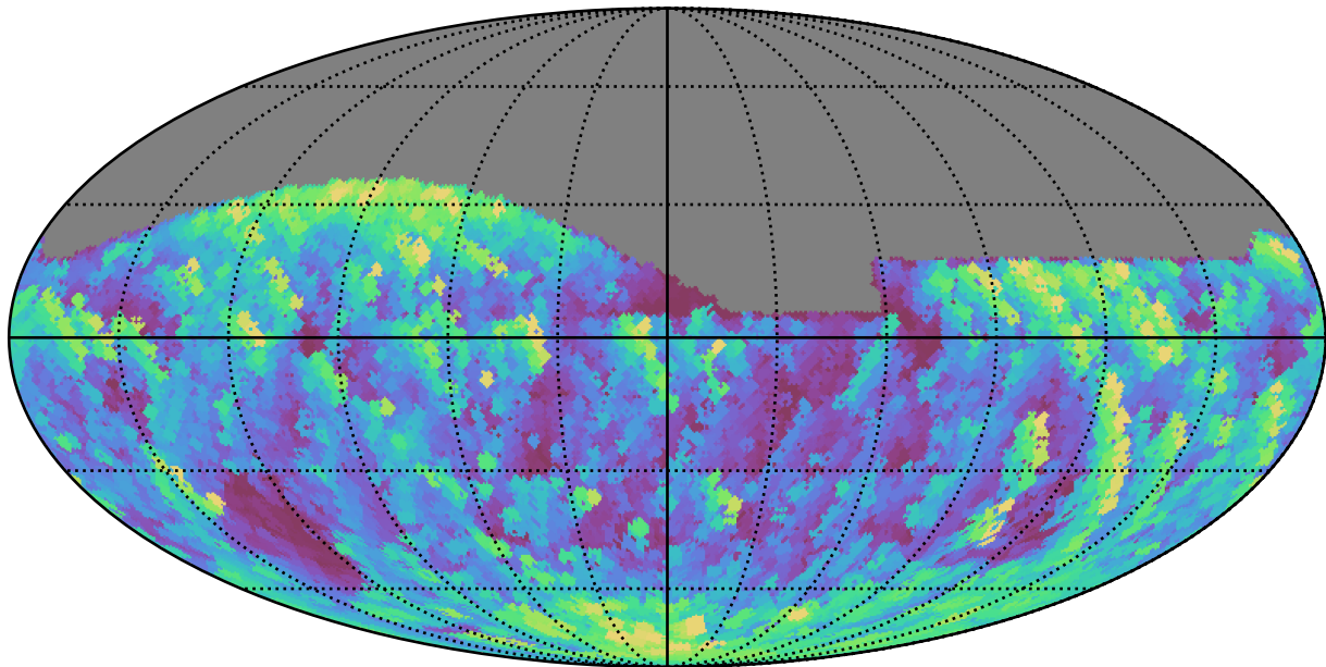
early_u_fpextra2.0_v3.4_10yrs All sky g band: Max airmass
